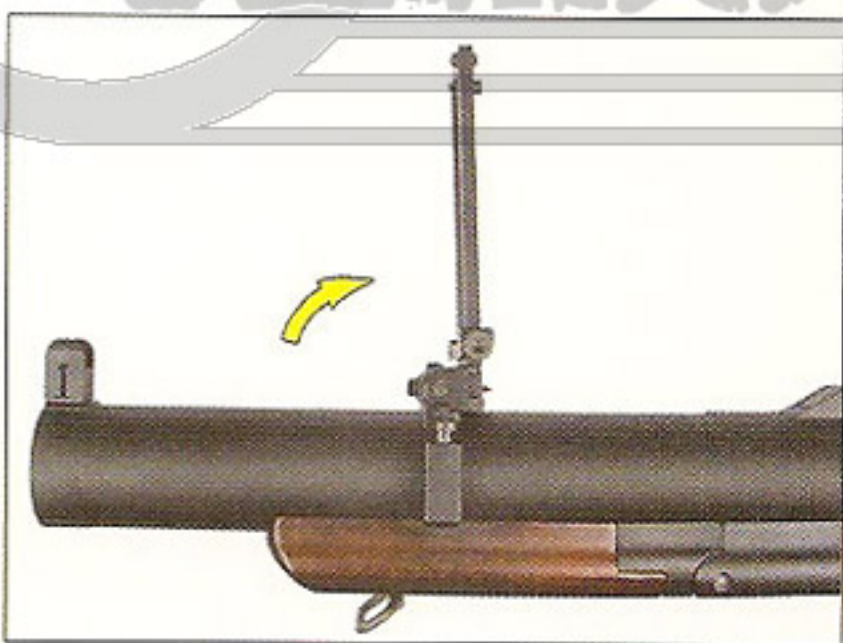
2. Push the button on the left side of the rear sight to unfold the folding ladder-style leaf-type sight. User can adjust the shooting range indicator by loosening the screw button. (Shooting range scale on indicator is not accurate for the Airsoft Version of the launcher.)
