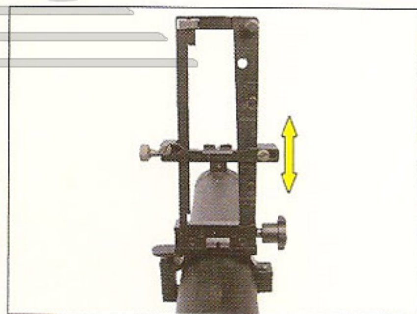
2. Push the button on the left side of the rear sight to unfold the folding ladder-style leaf-type sight. User can adjust the shooting range indicator by loosening the screw button. (Shooting range scale on indicator is not accurate for the Airsoft Version of the launcher.)
